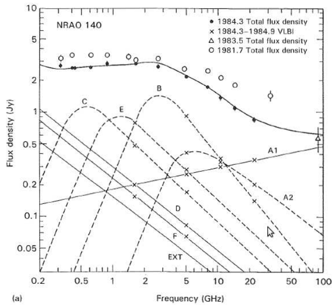
Figure 2.13: model of an accelerated jet (Marscher, 1996)
