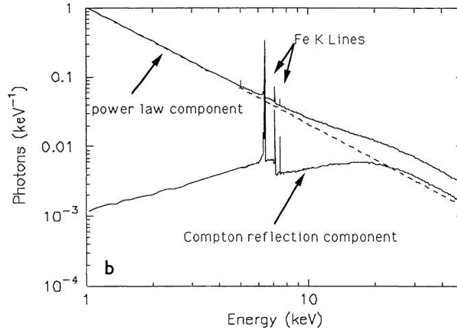
Figure 2.3: Theoretical X-ray spectrum, (George & Fabian, 1991) and (Mushotzky et al., 1993)
