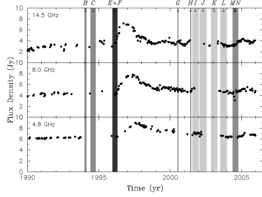
Figure 2.16: UMRAO Lightcurves of 3C111 (Kadler et al., 2008)
