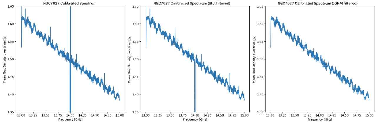
Figure 5.4: The mean flux density over time versus frequency is plotted for NGC7027 comparing two different types of filtering. The (left) plot depicts the calibrated spectrum without filtering. The (middle) plot the spectrum with the applied standard-deviation filter and the plot on the (right) has the IQRM filter applied. At around 13 GHz and 14 GHz there is interference that needs to be filtered out. The other protruding amplitudes represent the recombination lines of hydrogen and must not be removed by the filter.
