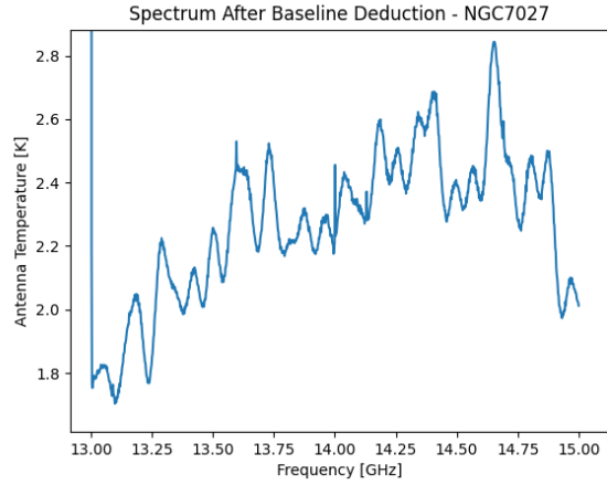
Figure 3.10: Mean flux density versus frequency for NGC7027 converted into antenna temperatures with deducted baselines for each frequency.
