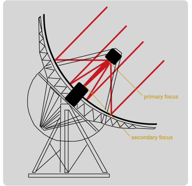
Figure 3.2: The path of incoming radiation for the Effelsberg 100m radio telescope is shown. The radiation is first bundled to the primary focus and then further into the secondary focus. Credit: based on https://www.mpifr-bonn.mpg.de/57598/exploring_universe
