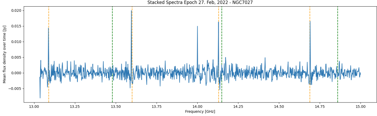
Figure A.1: Stacked calibrated spectra of NGC7027 for the Epoch of the 27. Feb, 2022 are shown. The over time integrated Flux Density is shown versus the Frequency. RFI below 13.1 GHz is removed, RFI at 14 GHz is visible. The calculated frequencies of recombination lines of hydrogen are marked in orange. Similar, the lines for positronium are marked as green dotted lines.
