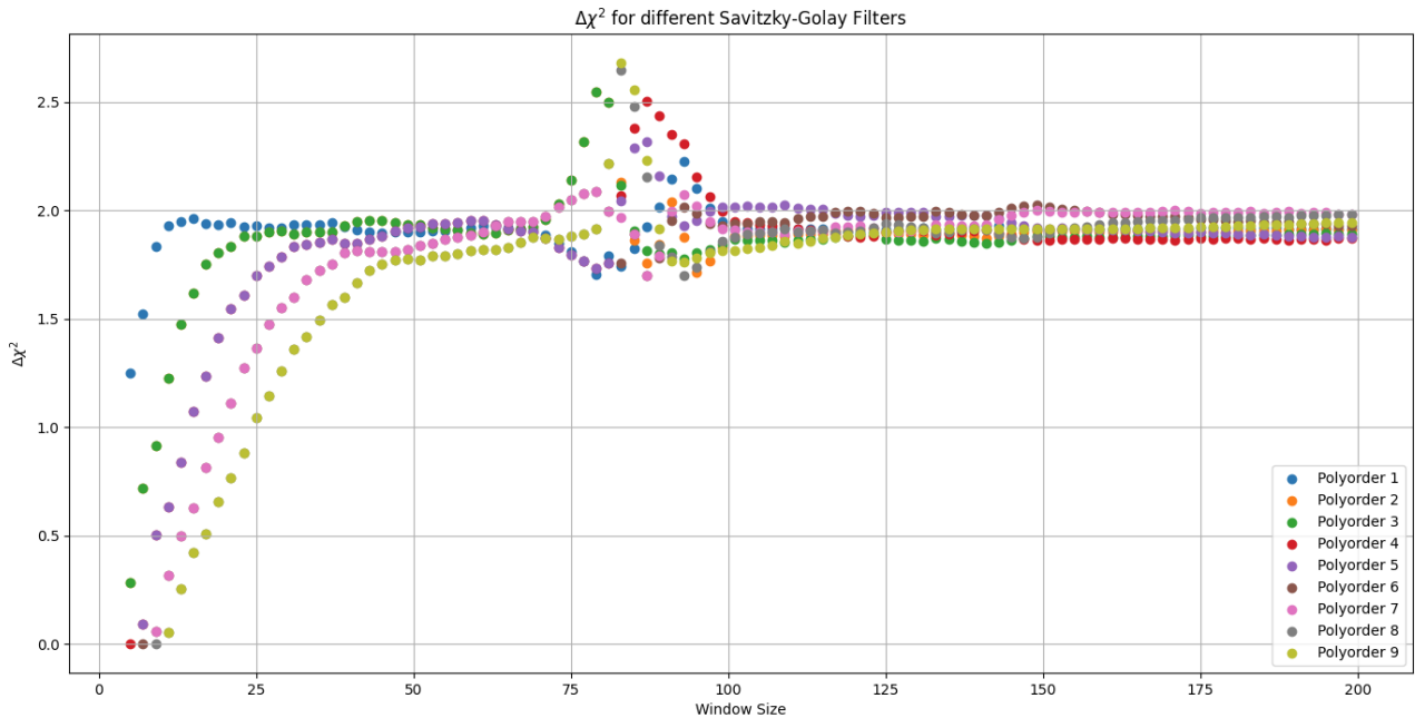
Figure 5.3: \Delta\chi^2 plotted versus window size, one of the two Savitzky-Golay parameters. The other parameter, represented by different colors, indicates the order of the fitted polynomial. The significant variation in \chi for a window size between 70 and 100 arises due to an outlier at the lower frequency edge. In this range, the outlier prevents a Gaussian fit to the H79 \alpha line, thereby distorting the results.
