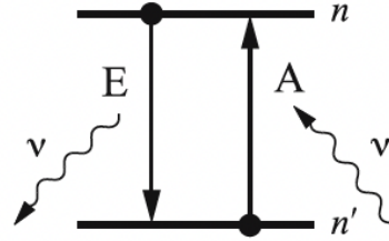
Figure 2.5: Energy transition of an electron from a higher energy level n to a lower level n' and vice versa. During the transition, a photon with frequency \nu is emitted or absorbed, accordingly. Credit: Leisi (2006)
