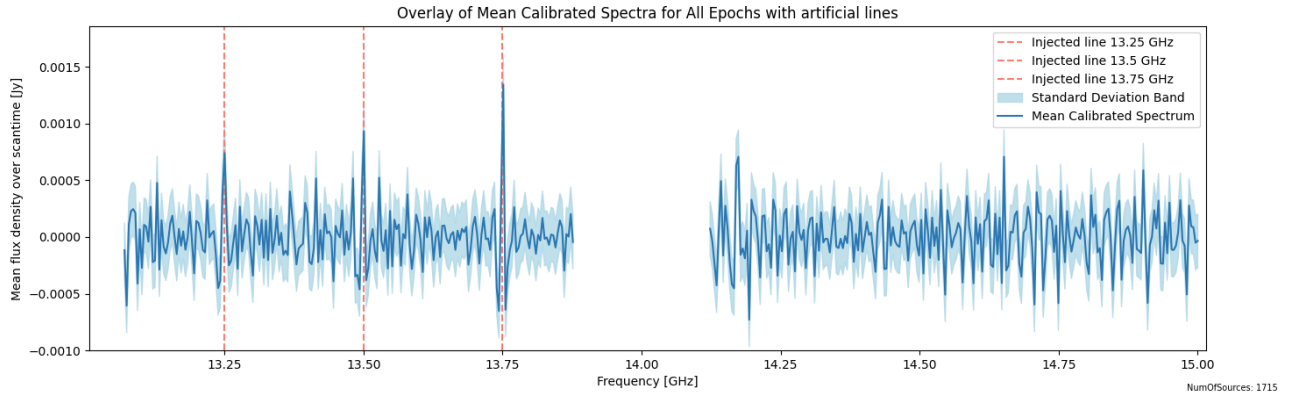
Figure 5.1: Mean calibrated spectrum of all overlaid target sources is plotted over the frequency. Before calibration three artificial recombination lines with a peak amplitude of 5 \times 10^5 counts ( <0.01 Jy) and width \sigma = 1 MHz are added at 13.25 GHz, 13.5 GHz and 13.75 GHz. Although these lines initially did not exceed the noise level, they become clearly visible after calibration. In order to preserve calibration accuracy, frequency ranges with higher interference, specifically 13–13.05 GHz and 13.9–14.1 GHz, were discarded.
