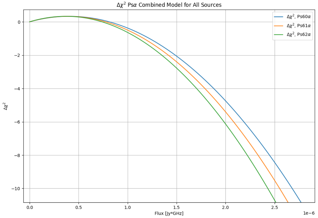
Figure A.5: \Delta\chi^2(F) plotted over the flux for all three expected positronium recombination lines within the frequency range of 13-15 GHz calculated with the "combined" method for all 1715 target scans overlaid. Comparing the two models \chi_0^2 (linear approximation) and \chi_1^2 (linear approximation with Gaussian added). The maxima of the curves represent the significance of the expected Ps\alpha lines.
