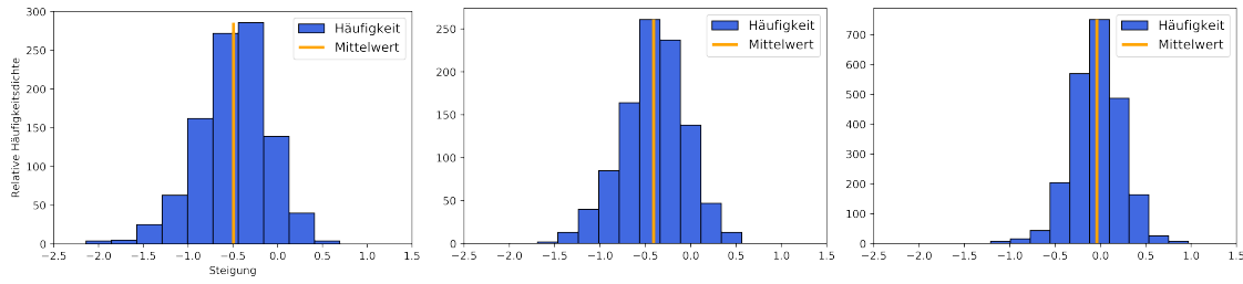
Fig. 5.9: Links: \mu = 5 , \sigma = 2 , mean_{5,2} = -0.494 \pm 0.189 , Mitte: \mu = 3 , \sigma = 1 , mean_{3,1} = -0.409 \pm 0.187 , Rechts: \mu = 1 , \sigma = 0.5 , mean_{1,0.5} = -0.040 \pm 0.183
