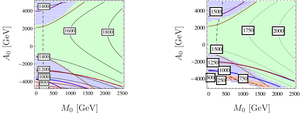
Figure 5.11.: Stop mass and vacuum stability in the (M_0, A_0) plane. We used M_{1/2} = 1 TeV, \mu > 0 and \tan \beta = 2 (left) or \tan \beta = 10 (right). The color coding is as in figure 5.4: points to the left of the solid lines fail the corresponding conditions. Again, there is a degeneracy between the more exclusive blue line of condition (4.10) with the dark red line of condition (4.7). Points to the left of the dashed line also have charged LSPs.
