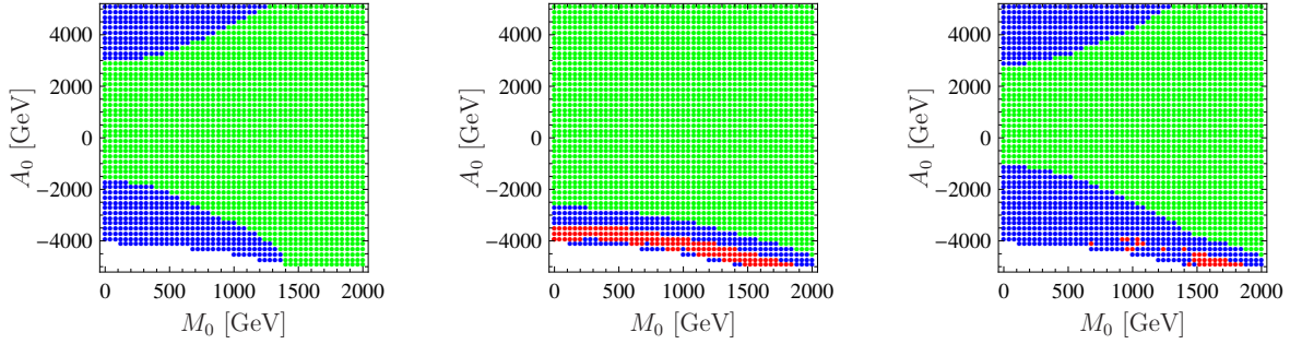
Figure 5.1.: Vacuum stability in the (M_0, A_0) -plane for input values of \tan \beta = 10 , M_{1/2} = 1 TeV and \mu > 0 . (Here and in the other figures, \tan \beta is taken to mean the input parameter for the DSB vacuum.) On the left, we allow only for stau VEVs, in the middle only for stop VEVs and on the right for both stau and stop VEVs. Green indicates that no CCB minimum deeper than the DSB minimum was found, while blue and red indicate that the DSB minimum is only metastable, as there is at least one deeper CCB minimum. The red points are short-lived, while the blue points are long-lived, compared to a threshold of three gigayears. The lack of a smooth boundary between red and blue is a numerical artifact and is discussed in the text.
