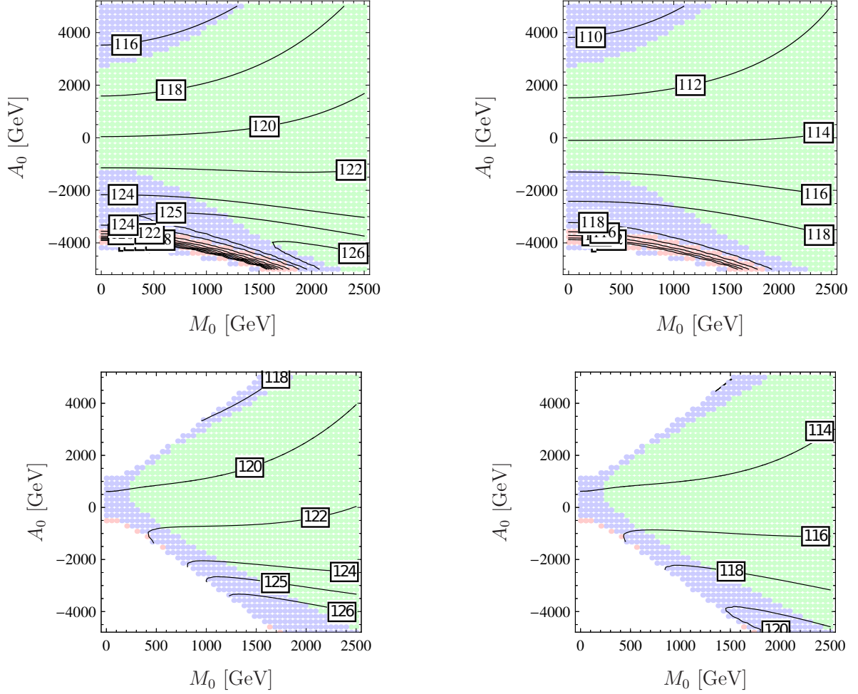
Figure 5.13.: Vacuum stability and the Higgs mass in the (M_0, A_0) plane for fixed M_{1/2} = 1 TeV, \mu > 0 and \tan \beta = 10 (upper) or \tan \beta = 40 (lower). On the left, the leading two-loop corrections to the mass of the lighter Higgs boson have been taken into account, on the right, only the mass at one-loop order is shown. The color coding is the same as in figure 5.1.
