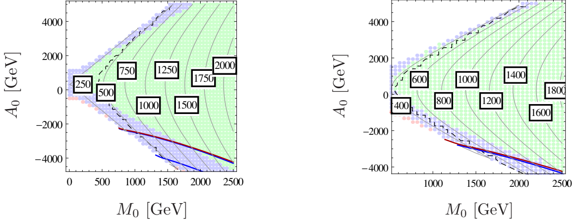
Figure 5.8.: Vacuum stability and stau masses in the (M_0, A_0) plane for fixed M_{1/2} = 1 TeV, \mu > 0 and \tan \beta = 40 (left) or \tan \beta = 50 (right). The dashed black line shows the transition to a charged LSP (neutralino LSP to the right of the line). The color coding is as in figure 5.4: points to the left of the solid lines fail the corresponding conditions. As in figure 5.7, the blue line for condition (4.10) with 0.65^2 is almost degenerate with the dark red line of condition (4.7) and the line for 0.85^2 only excludes points with even more negative A_0 (and is not visible on the right).
