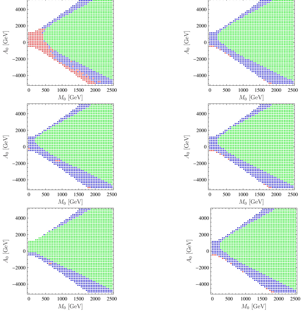
Figure 5.2.: Vacuum stability in the (M_0, A_0) -plane for fixed M_{1/2} = 1 TeV, \mu > 0 and \tan \beta = 40 . On the left, only the tree level potential was considered. On the right, the full one-loop effective potential was taken into account. The renormalization scale was Q = \sqrt{m_{\tilde{t}_1} m_{\tilde{t}_2}}/2 (first row), Q = \sqrt{m_{\tilde{t}_1} m_{\tilde{t}_2}} (second row), and Q = 2\sqrt{m_{\tilde{t}_1} m_{\tilde{t}_2}} (last row). The color code is the same as in figure 5.1.
