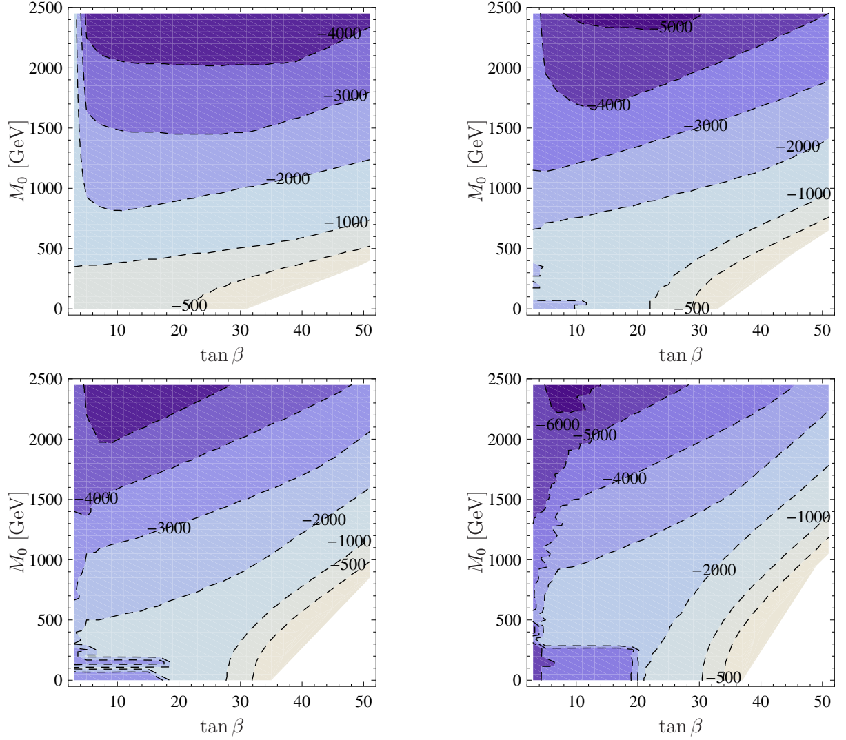
Figure 5.3.: Minimal value allowed for A_0 in the (\tan \beta, M_0) plane to have a stable DSB vacuum. We used \mu > 0 and M_{1/2} = 500 GeV (upper left), M_{1/2} = 1000 GeV (upper right), M_{1/2} = 1500 GeV (lower left) and M_{1/2} = 2000 GeV (lower right).
