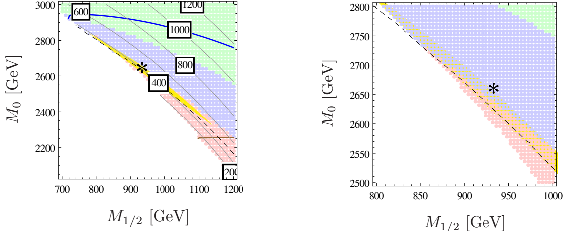
Figure 5.10.: Mass of the light stop and vacuum stability in the (M_{1/2}, M_0) plane with A_0 = -6444 GeV, \mu < 0 and \tan \beta = 8.52 . The dashed line shows the transition to a charged LSP (neutralino LSP to the right of the line). The color coding is as in figure 5.4: points below the solid lines fail the corresponding conditions. In the yellow region, \Omega h^2 is in agreement with dark matter constraints (as in figure 5.7). The star indicates the benchmark point 5.1 of [121]. The reason that this point is not in the strip with the correct dark matter abundance is that different SM input parameters were used in [121] in comparison to eq. (5.1): m_t = 174.3 GeV, \alpha_S = 0.1172 and m_b(m_b) = 4.25 GeV. The line showing the division between passing and failing condition (4.10) using 0.65^2 does not appear on this plot, but over-zealously would exclude the entire region shown, while taking 0.65^2 would only exclude every point with M_0 \lesssim 2900 GeV.
