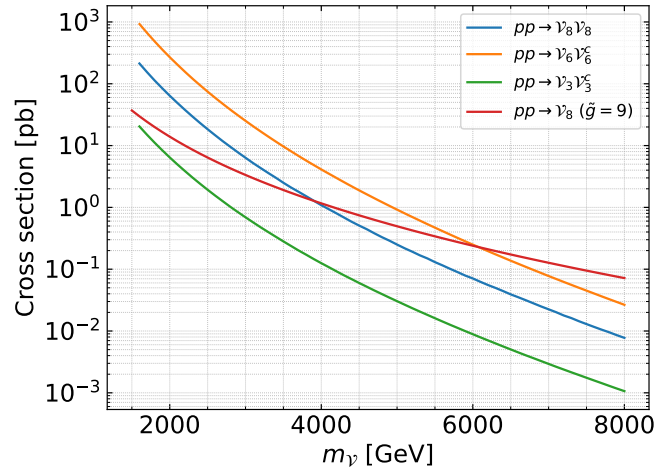
Figure 6.7: Pair production cross section of spin-1 resonances at a \sqrt{s} = 100 TeV pp -collider. The values also apply to axial vectors. For comparison we show the single production cross section for \tilde{g} = 9 .
