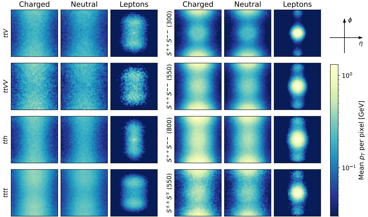
Figure 4.19: Distribution of jet and lepton images of (left) background and (right) signal processes, where the scalar mass in GeV is given in parentheses. The final state signatures are discretised into 50 \times 50 calorimeter grids within a region of -2.5 \leq \eta \leq 2.5 and -\pi \leq \phi \leq \pi . The origin of the coordinate system is the centre of the two same-sign leptons. The columns show charged and neutral components of the jets, as well as isolated leptons, respectively. The colourbar indicates the mean p_T per pixel.
